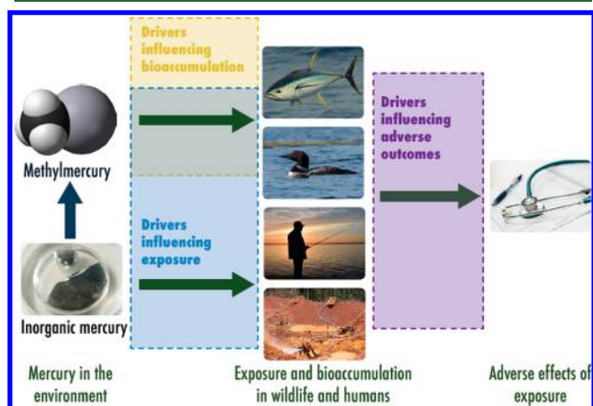
Figure 4. Biological, ecological, and socioeconomic drivers that influence mercury accumulation, exposure, and adverse effects. Drivers influencing bioaccumulation and exposure overlap for fish and wildlife (gray box). Adapted with permission from ref 3. Copyright 2018 Eagles-Smith et al. ( http://creativecommons.org/licenses/by/4.0/ ).
