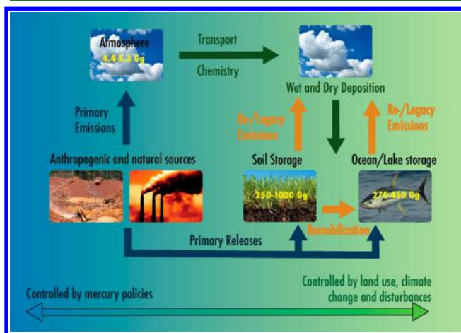
Figure 2. Atmospheric mercury influenced by new emissions, and recycling of legacy mercury in sources and sinks on land and in oceans. Releases of mercury to the environment (blue), mercury transport (green), mercury recycling (orange), mercury quantity in each reservoir in gigagrams (yellow). Note that dry mercury deposition includes the deposition of mercury associated with vegetation uptake. Adapted with permission from ref 1. Copyright 2018 Obrist et al. ( http://creativecommons.org/licenses/by/4.0/ ).
